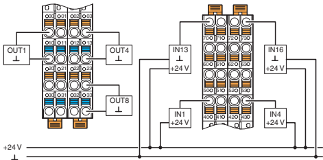
Connection example
