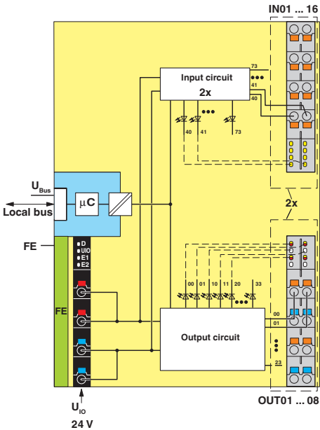
Block diagram
